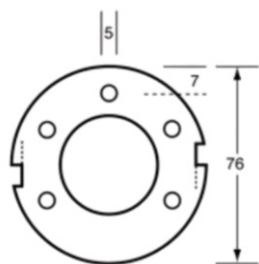
MODEL BTR-01-014 Rear view
