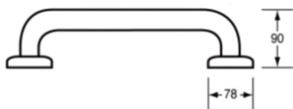
MODEL BTR-01-014 Side view
