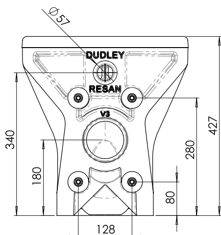
MODEL BSSP-WF-G Rear View
