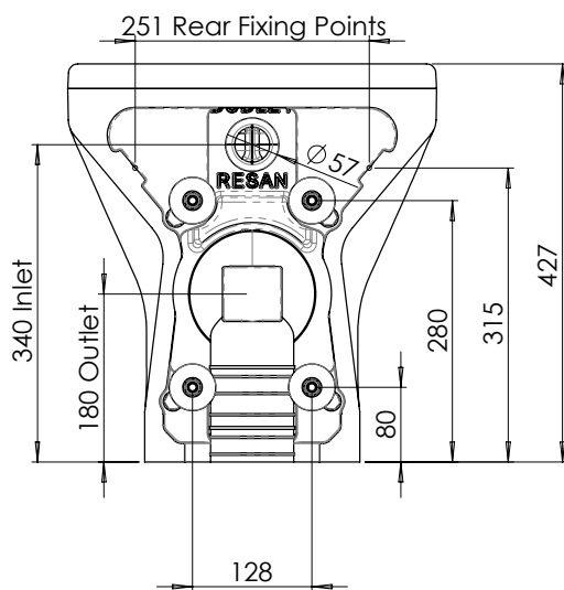
MODEL BSSP-FW-G Rear View
