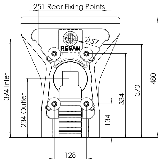
MODEL BSSP-AM-G Rear View
