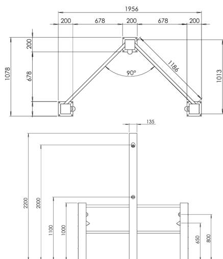
MODEL BQBS-3 Plan and Front view
