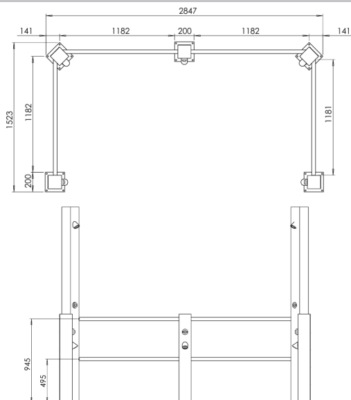
MODEL BQBS-5 Plan and front view
