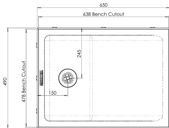
MODEL BB1 Plan View
