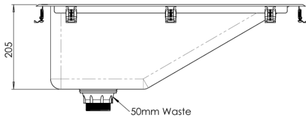
MODEL BB1 Side View
