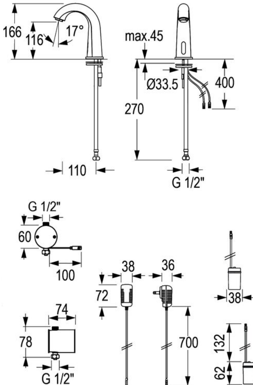
MODEL AESB/AESB-B Side & Front View
